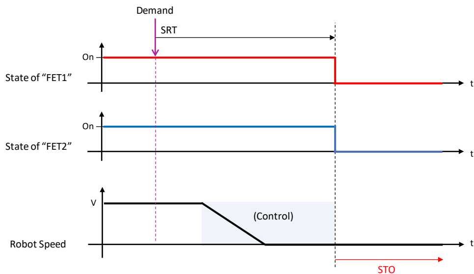
Fig. 1 Safety function response time of Safe stop 1
